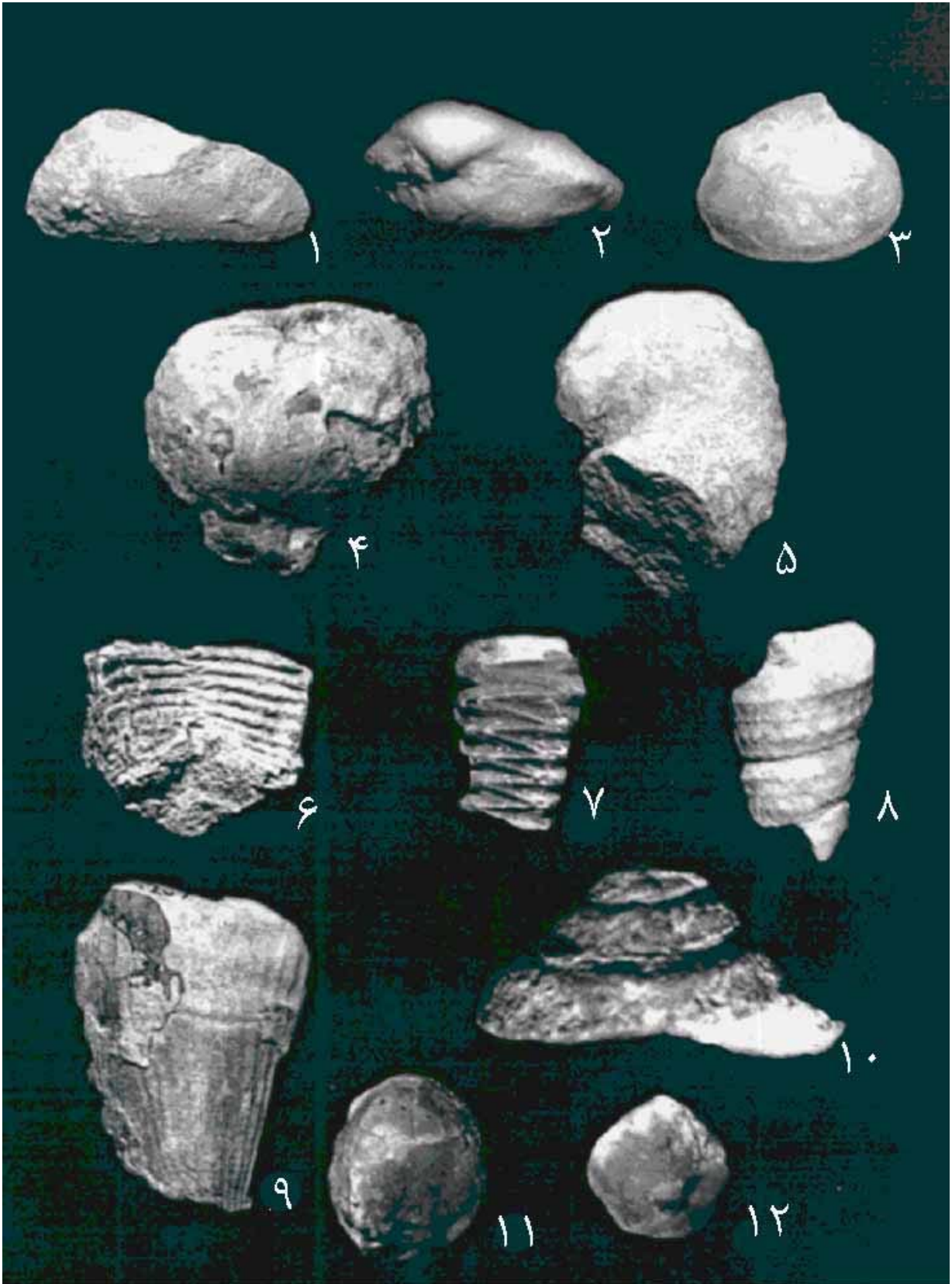
Venerid bivalve Panopea sp. : Pinna decussata Goldfuss Turritella sp. Rastellum (Acrostrea) sp. Sponge Siphonia sp. Astartid bivalve Gibbithyris sp. Unidentified brachiopod Pleurotomaria sp.
