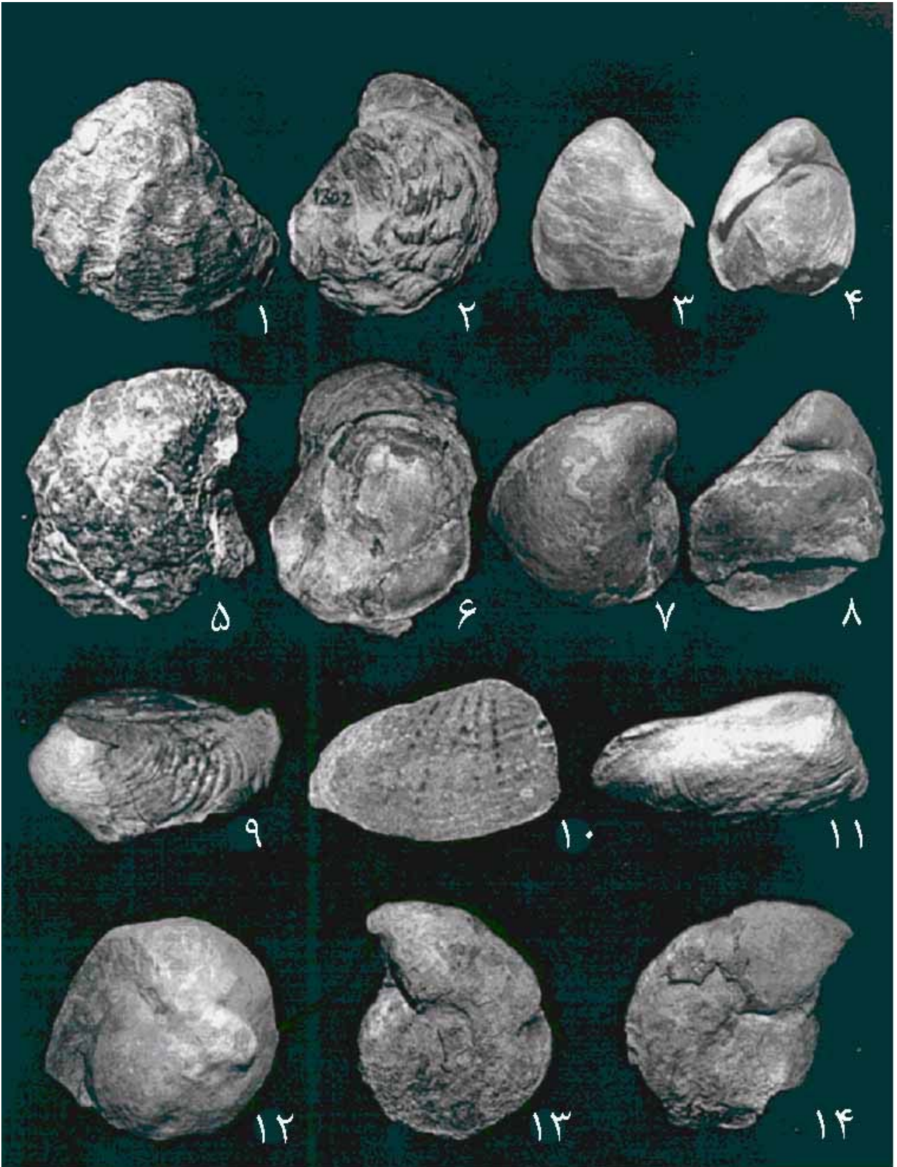
Exogyra olisiponensis Sharpe : Tissotia Pholadomya spp. Exogyra sp. Exogyra cf. olisiponensis Sharpe Exogyra mermeti Albano Heterotissotia sp. ( subtissotia ) sp.
