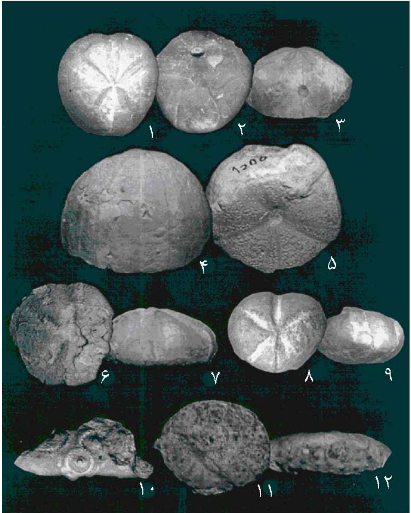
Conulus Pliotoxaster sp. : Micraster sp. Hemiaster syriacus (Conrad) carcharicus Cotteau Tetragramma Temnocidaris sp. variolare (Brongniart)
