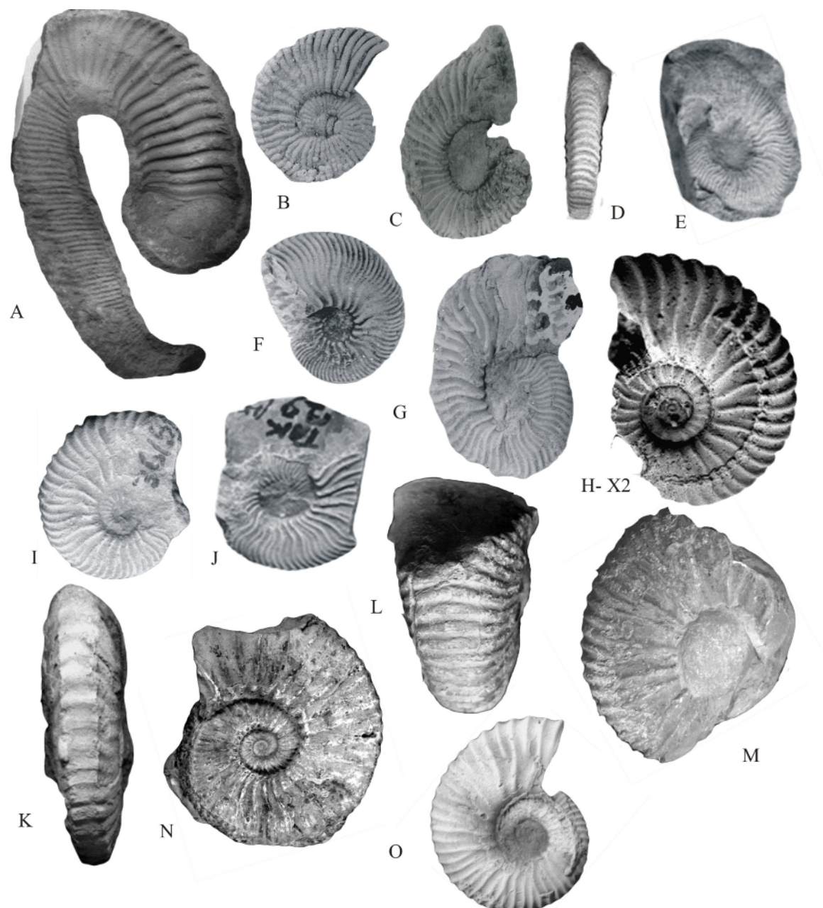
A- Heteroceras cf. colchicus , Sarcheshmeh Formation, Takal Kuh section B- Martelites cf. tinae , Sarcheshmeh Formation, Takal Kuh section C& D- Martelites cf. scuriformis , Sarcheshmh Formation, Takal Kuh section E- Deshayesites cf. tuarkyricus , Sarcheshmeh Formation, Takal Kuh section F- Deshayesites oglanlensis , Sarcheshmeh Formation, Takal Kuh section G- Deshayesites weissi , Sarcheshmeh Formation, Takal Kuh section H & I- Deshayesites deshayesi , Sarcheshmeh Formation, Takl Kuh section J- Deshayesites cf. planus , Sarcheshmeh Formation, Takal Kuh section K- Dufrenoyia sp., Sarcheshmeh Formation, Raz section L & M- Parahoplites cf. campichii , Sanganeh Formation, Sanganeh section N- Hypacanthoplites uhligi , Sanganeh formation, Bibahre section O- Acanthohoplites cf. aschiltaensis , Sanganeh Formation, Sanganeh section
